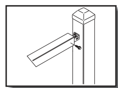
INTERNAL "L"-CLIP
